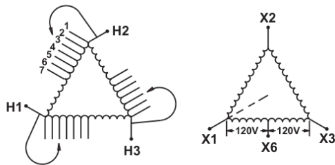
Schematic
